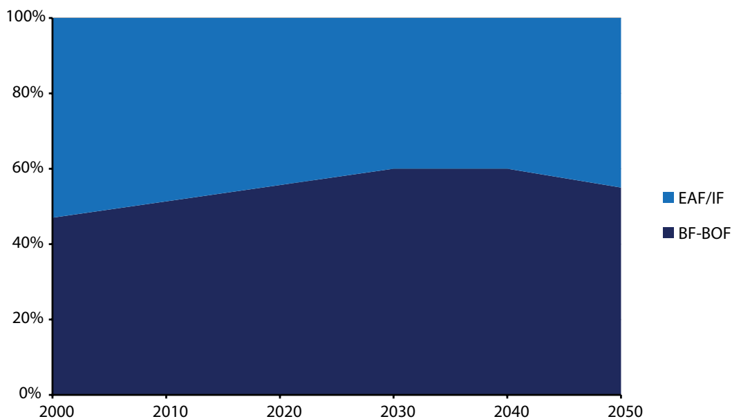
Figure 22: Production route shares by technology, 2000–50
