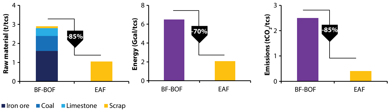
Figure 16: Material, energy and emissions benefits of scrap-based production
