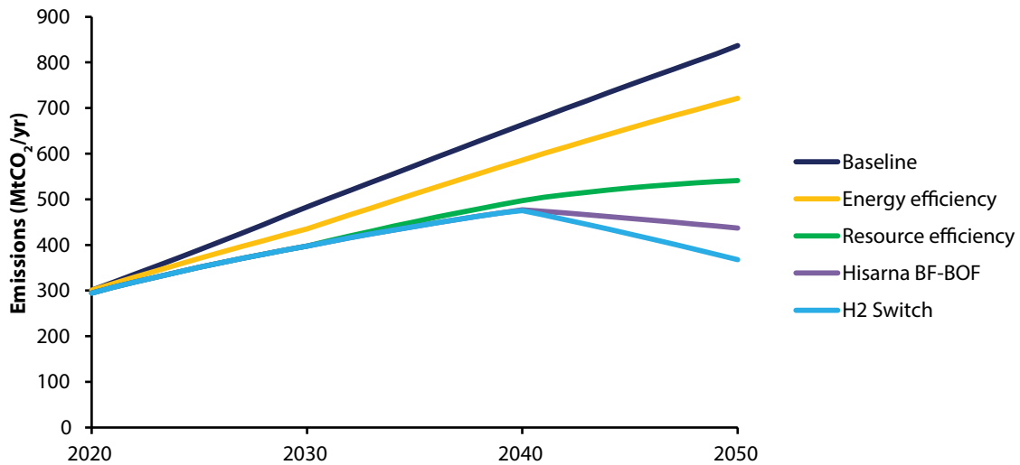
Figure 50: Deep decarbonization pathway for the iron and steel sector
