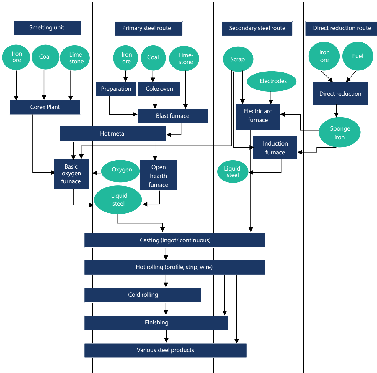
Figure 1: Steel production routes
