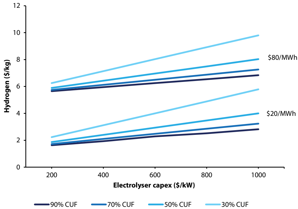
Figure 52: Impact of varying capacity utilization factors (CUF) on cost of hydrogen
