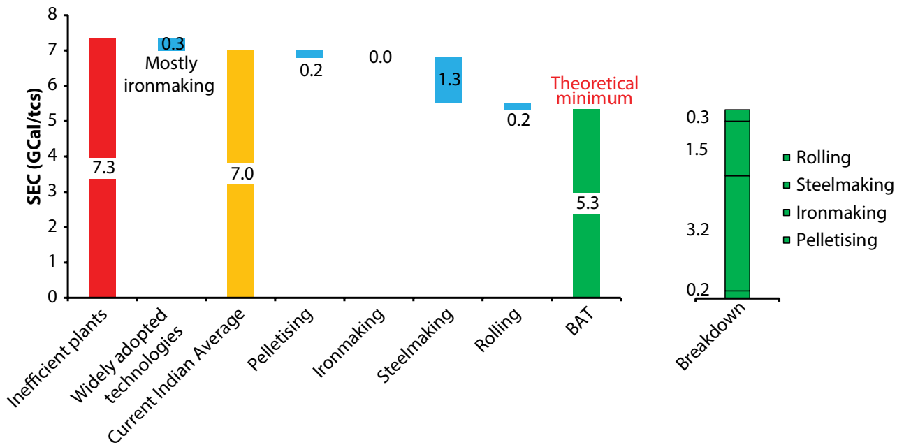
Figure 25: Energy efficiency measures for the coal-based DR-EAF/IF route
