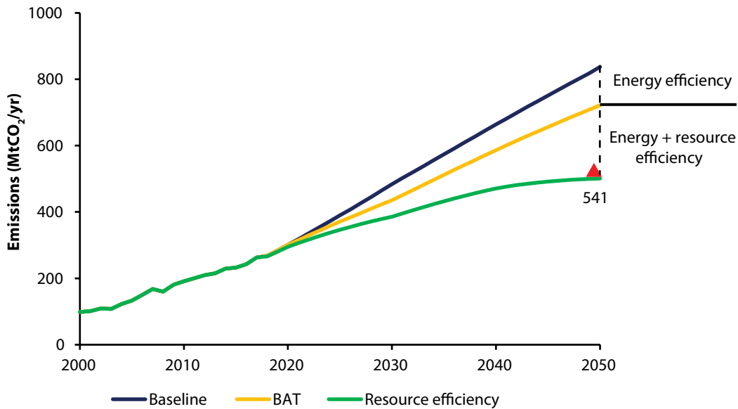
Figure 28: Emissions impact of energy efficiency and resource efficiency
