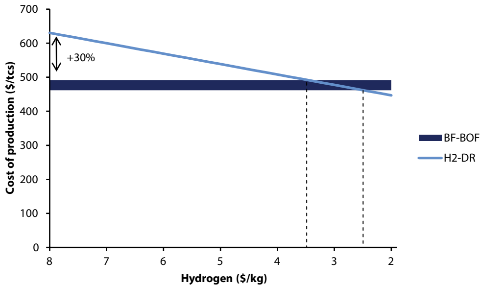
Figure 53: Cost of H2-DR versus BF-BOF for greenfield sites
