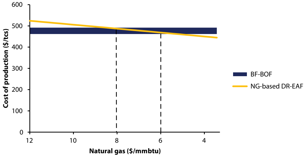
Figure 44: Costs of steel production from greenfield BF-BOF and gas-based DR-EAF plants at different natural gas prices
