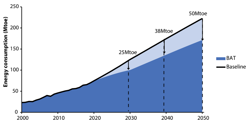
Figure 26: Energy consumption impact efficiency measures, 2000–50
