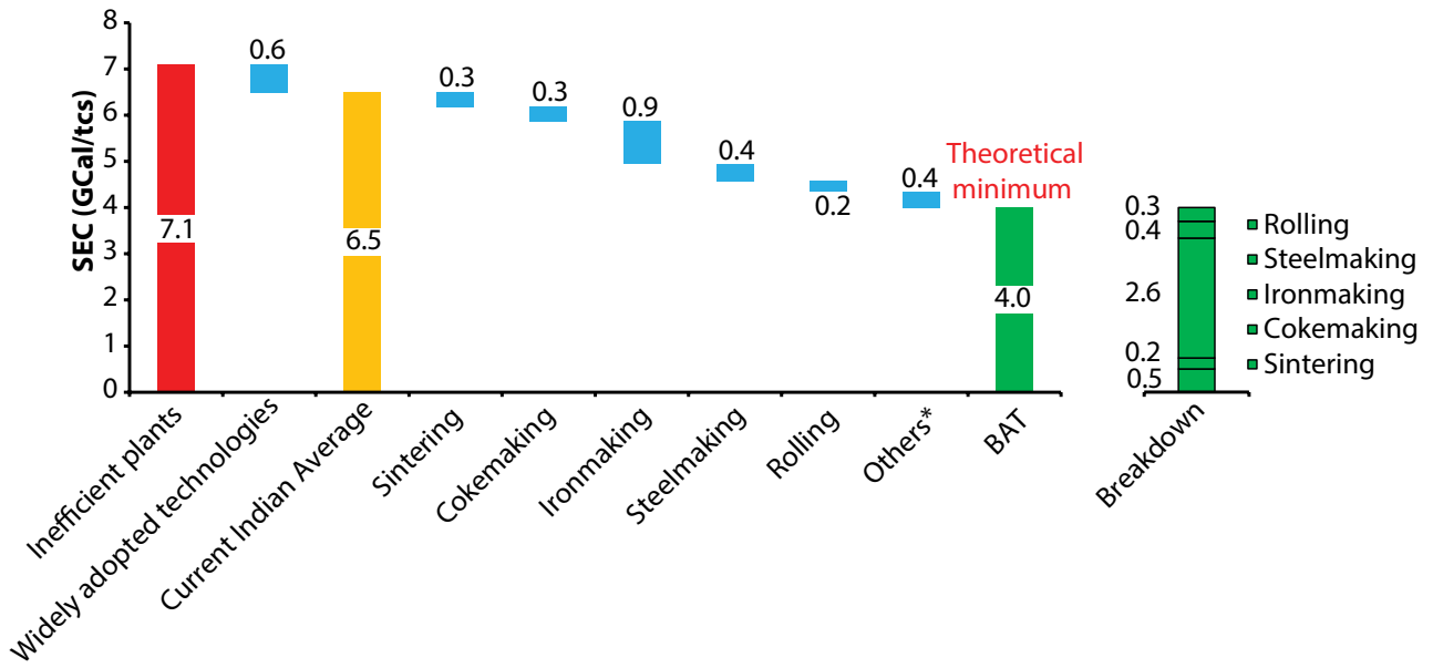
Figure 24: Energy efficiency measures for the BF-BOF route
