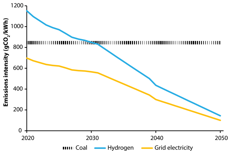
Figure 47: Emissions intensity of electricity and hydrogen, 2020–50
