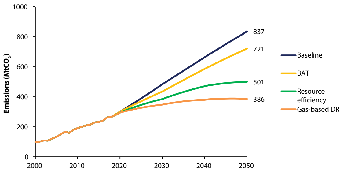
Figure 45: Emissions impact of coal to gas switch in DR facilities, 2000–50
