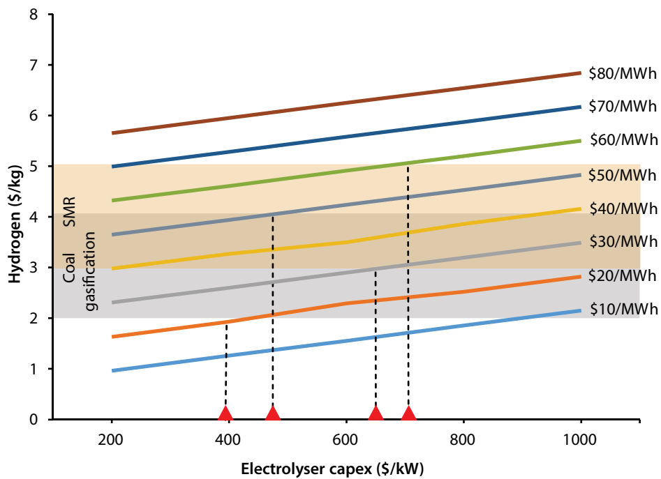
Figure 51: Costs of hydrogen from electrolysis
