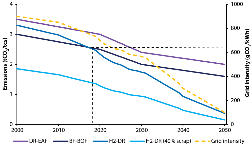
Figure 48: Emissions of different steelmaking routes
